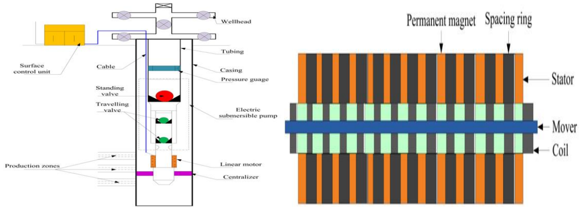
Fig.(1) Schematic diagram of the reciprocating direct-drive electric submersible plunger pump lifting system.
